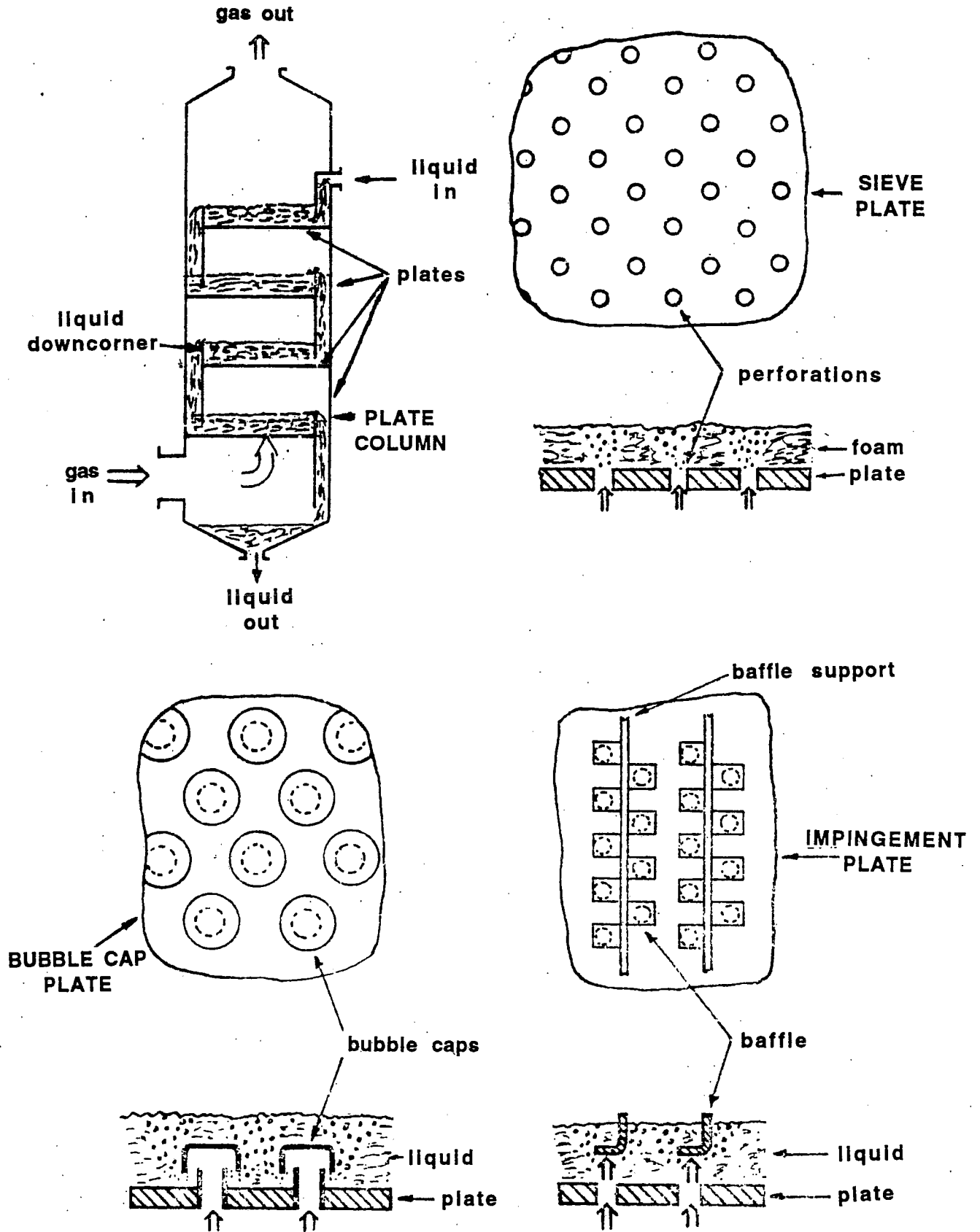
Figure III-1. Plate Scrubbers
