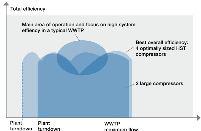
Four optimally sized HST compressors achieve better turndown.
