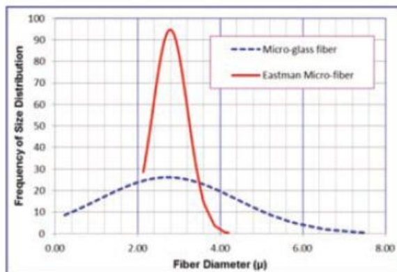
Figure 1: Eastman Cyphrex 10001 diameter distribution, determined by utilizing scanning electron microscopy (SEM) and compared with a commercial microglass of comparable average diameter.
