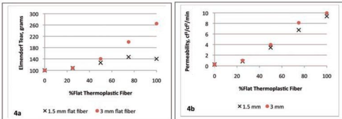
Figures 4a and 4b: Tear strength and permeability of 80 gsm handsheets as a function of softwood Kraft cellulose fiber (50 Schopper-Riegler) and flat thermoplastic fiber content.
