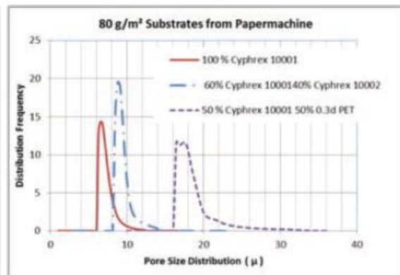
Figure 2: Pore size distribution profiles of 80 gsm nonwoven substrates produced on a commercial wetlaid machine.
