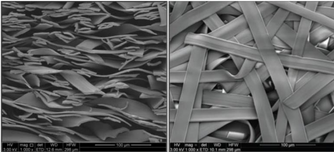
Figure 3: SEM images (side and top views, from left to right) of a wetlaid nonwoven media composed of developmental, flat thermoplastic microfibrer.
