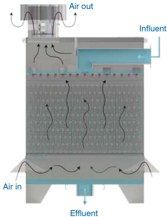
Induced Draft Aerator Process Flow Diagram
