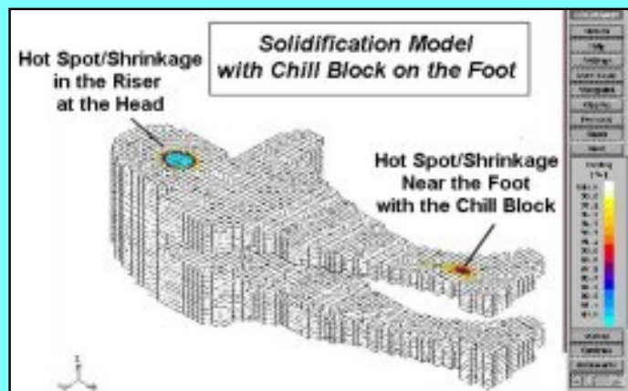
Solidification Model
